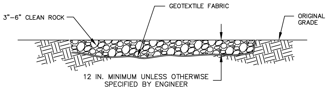
SECTION B-B
