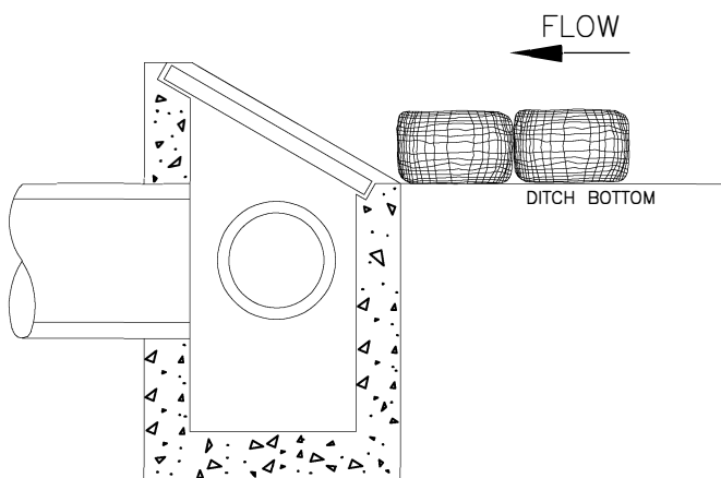
CATCH BASIN
