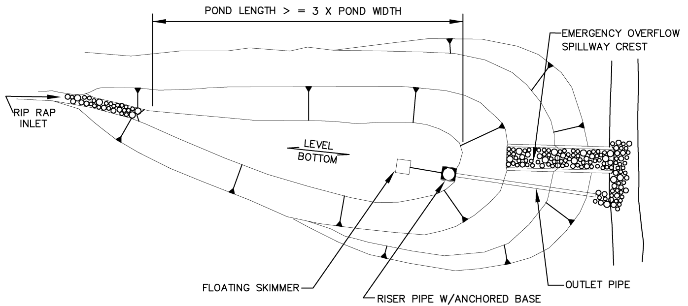
PLAN VIEW
