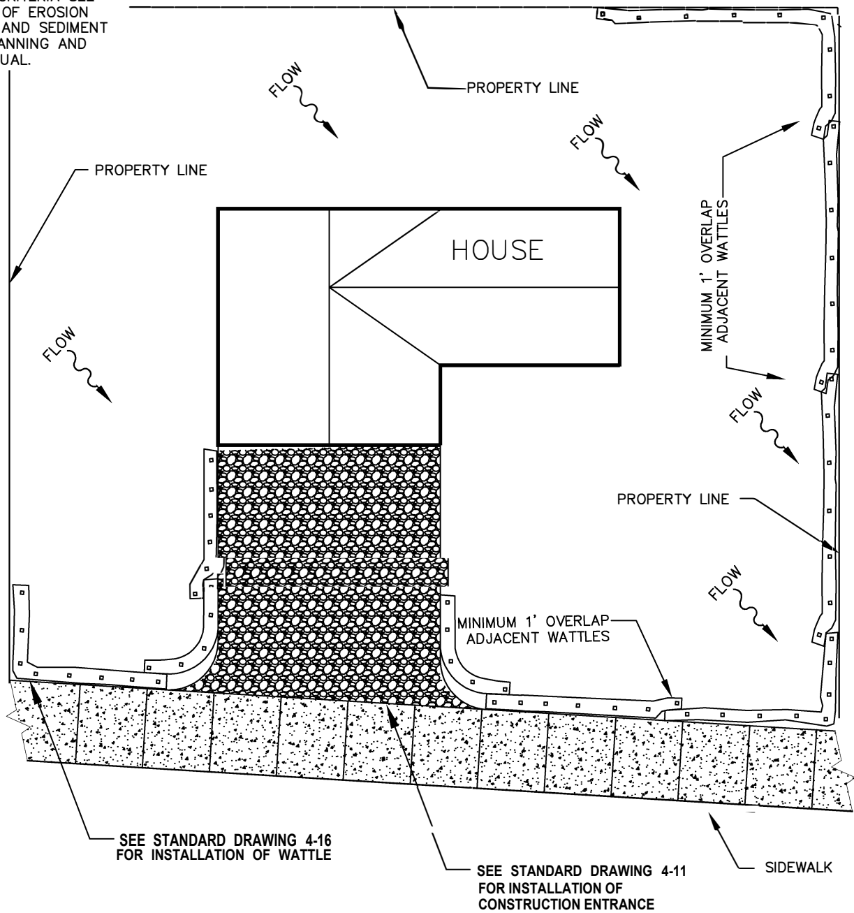
PLAN VIEW
