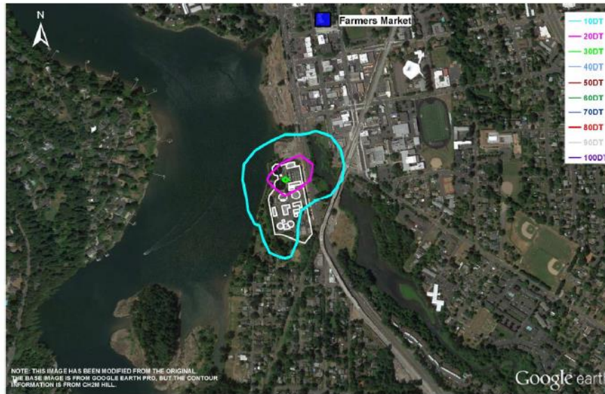
Alternative D4: Cover and treat just inlet portion of ABs (Clarifier Source not shown)
