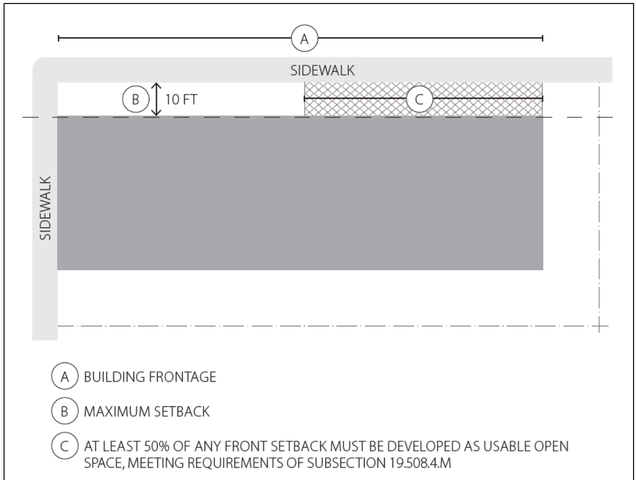
Figure 19.508.4.A.2.b.(2) Maximum Setbacks
