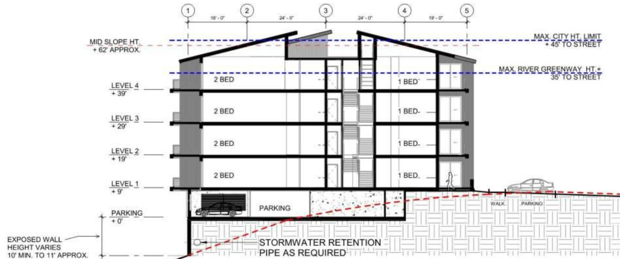
1 BUILDING A.1 (A.2 SIM) - SECTION DIAGRAM --- EXISTING TOPOGRAPHY
