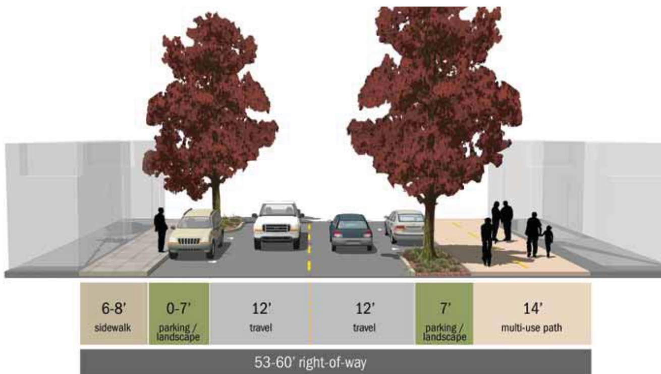
Figure 17. Conceptual Cross-Section for Main Street North of Beta Street (looking north)
