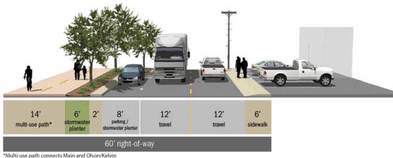
Figure A-10. Conceptual Cross-Section for Mailwell Drive with continuous access (looking east)
