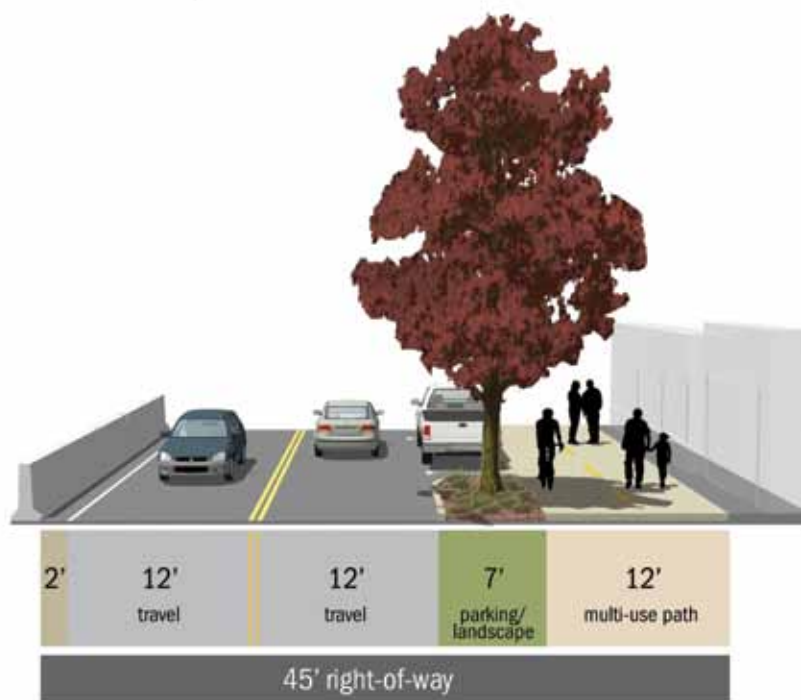
Figure A-2. Conceptual Cross-Section for Main Street – Milport Road to Beta Street within existing right-of-way (looking north)
