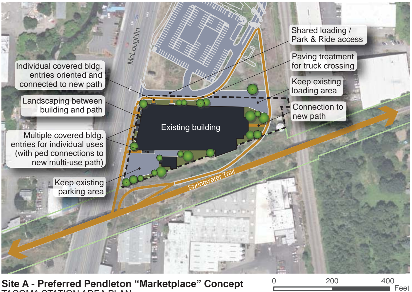
Figure 2. Conceptual Site Plan for Redevelopment of Opportunity Site A
