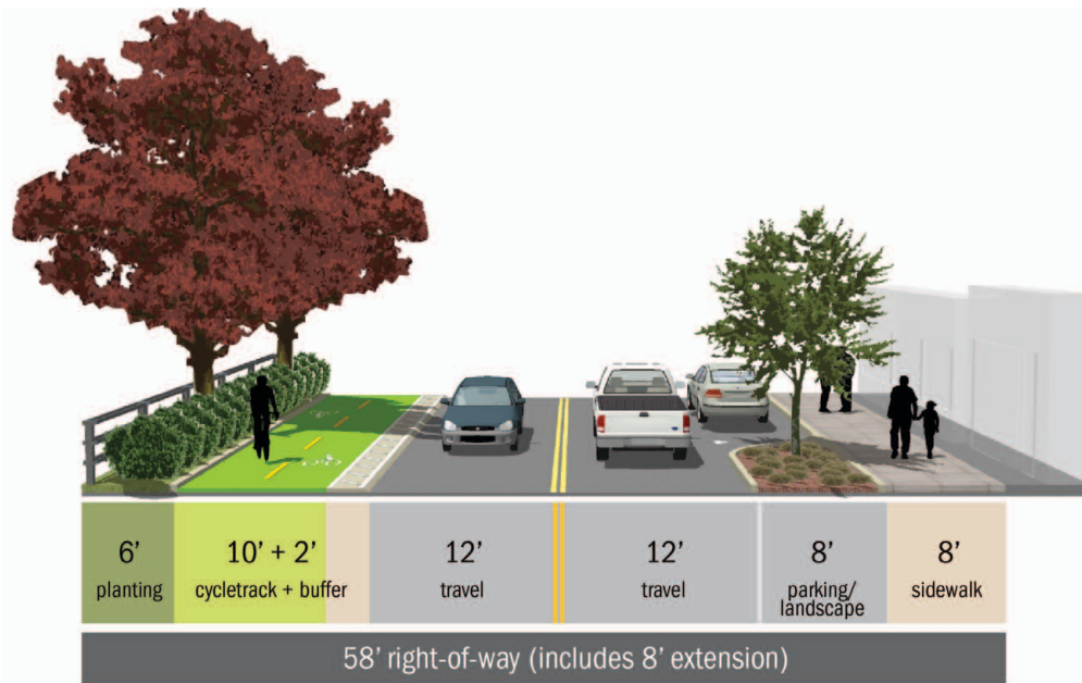
Figure A-5. Conceptual Cross-Section for Main Street – Milport Road to Beta Street with additional right-of-way and Cycletrack
