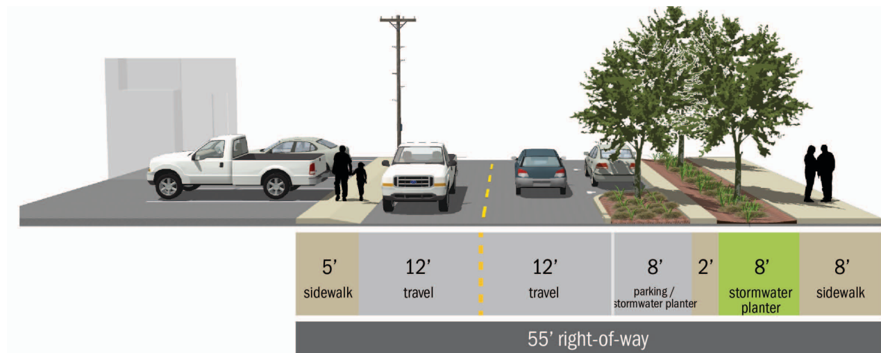
Figure A-15. Conceptual Cross-Section for Stubb Street with continuous access
