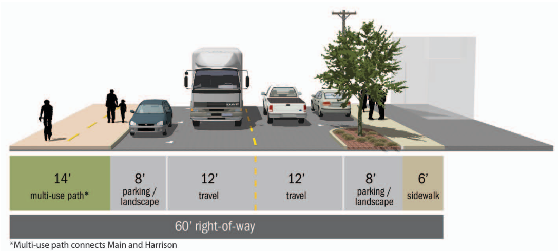
Figure A-14. Conceptual Cross-Section for Mailwell Drive with on-street parking
