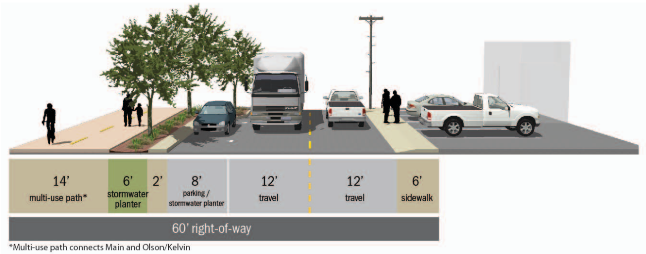
Figure A-13. Conceptual Cross-Section for Mailwell Drive with continuous access
