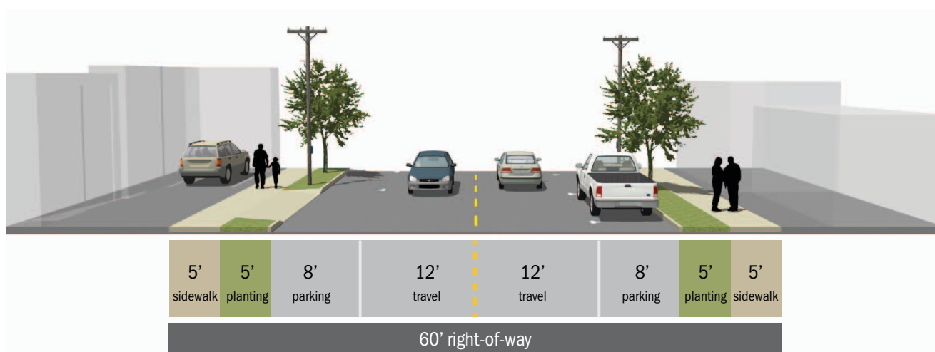
Figure A-16. Proposed Conceptual Cross-Section for General Industrial Streets South of Mailwell Drive
