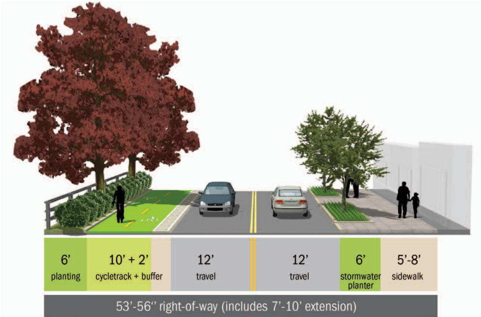
Figure A-3. Conceptual Cross-Section for Main Street – South of Milport Road with additional right-of-way and Cycletrack
