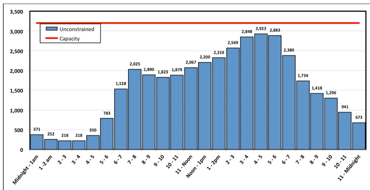
Figure 7: 24-hour weekday Duration of Congestion profile, McLoughlin Boulevard southbound north of Ochoco Street
