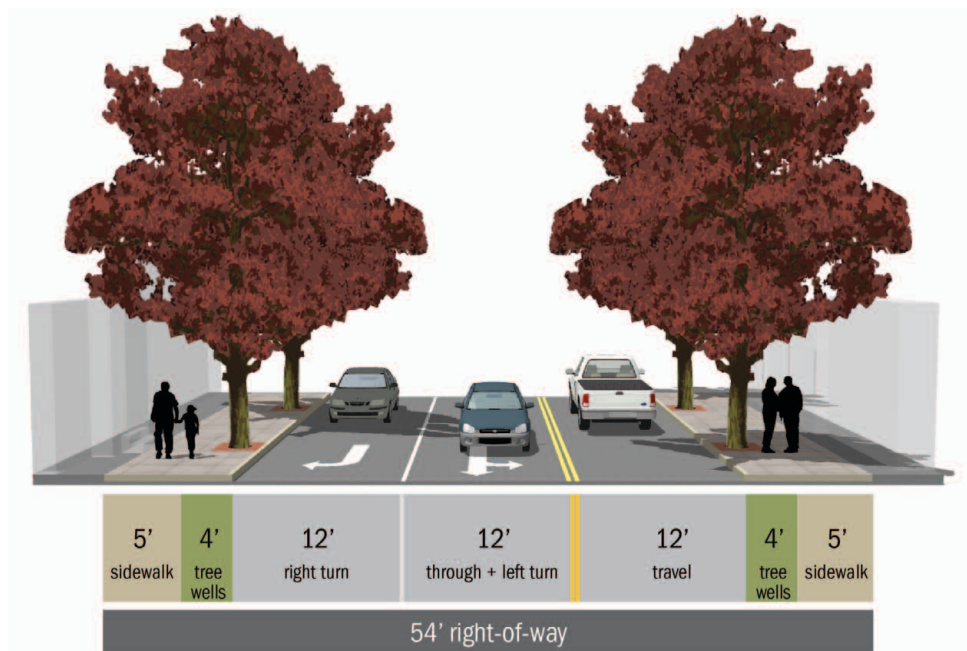
Figure A-8. Conceptual Cross-Section for Ochoco Street – West of Main Street within existing right-of-way
