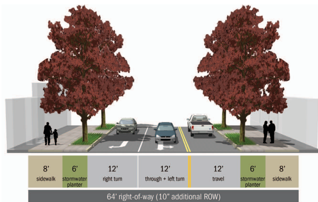
Figure A-9. Conceptual Cross-Section for Ochoco Street – West of Main Street with additional right-of-way
