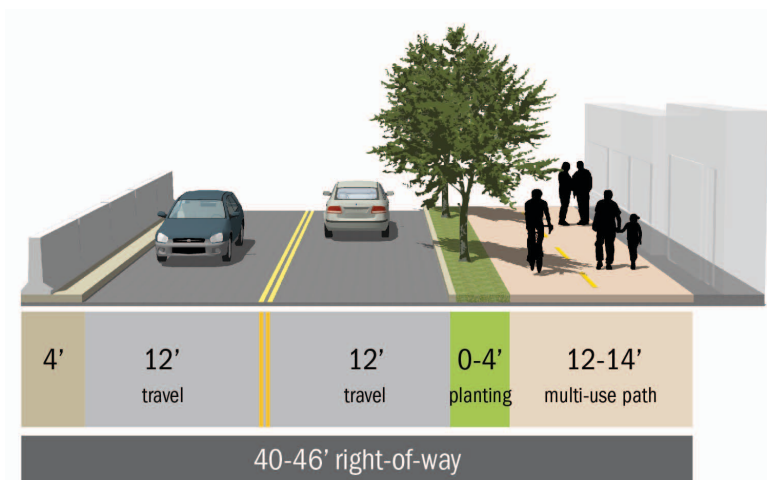
Figure A-1. Conceptual Cross-Section for Main Street – South of Milport Road within existing right-of-way
