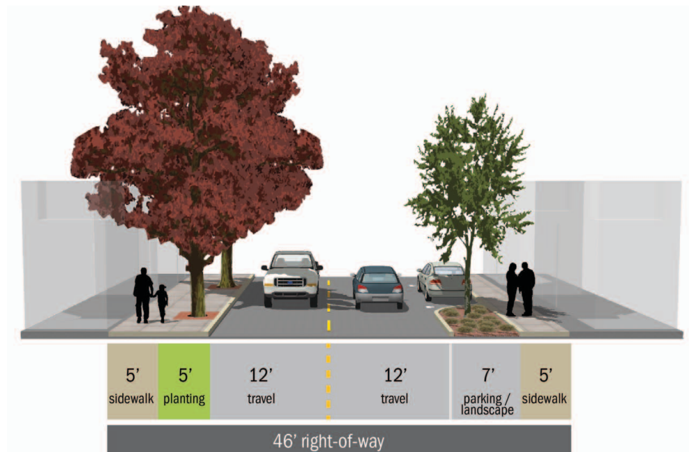
Figure A-6. Conceptual Cross-Section for Main Street – North of Beta Street within existing right-of-way
