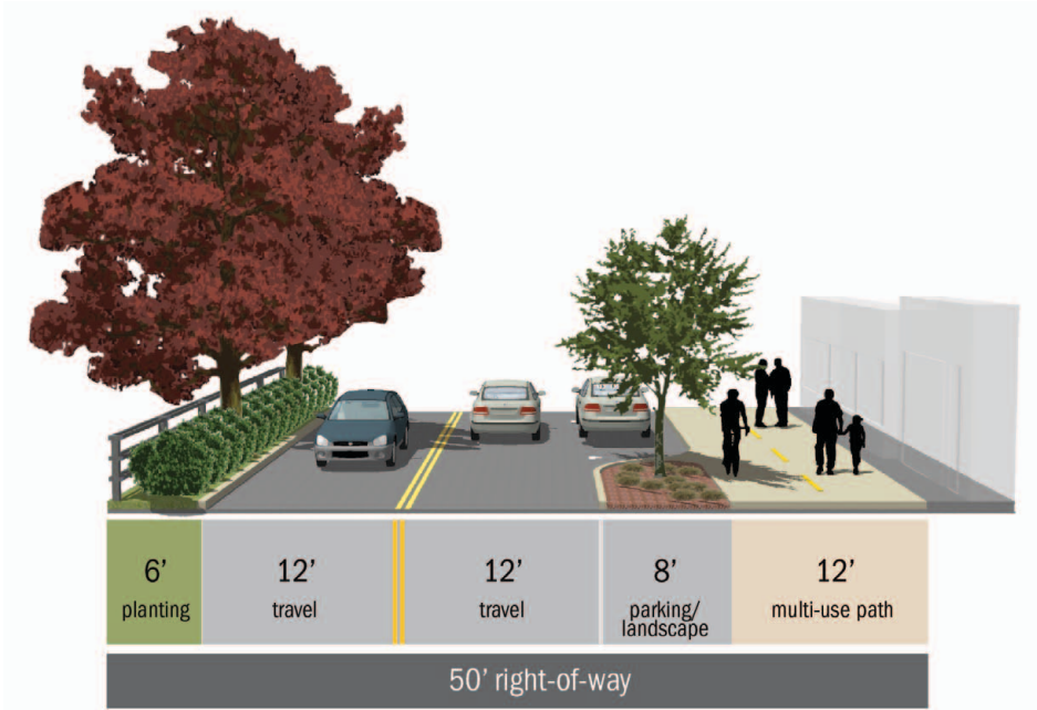
Figure A-4. Conceptual Cross-Section for Main Street – Milport Road to Beta Street with additional right-of-way and multi-use
