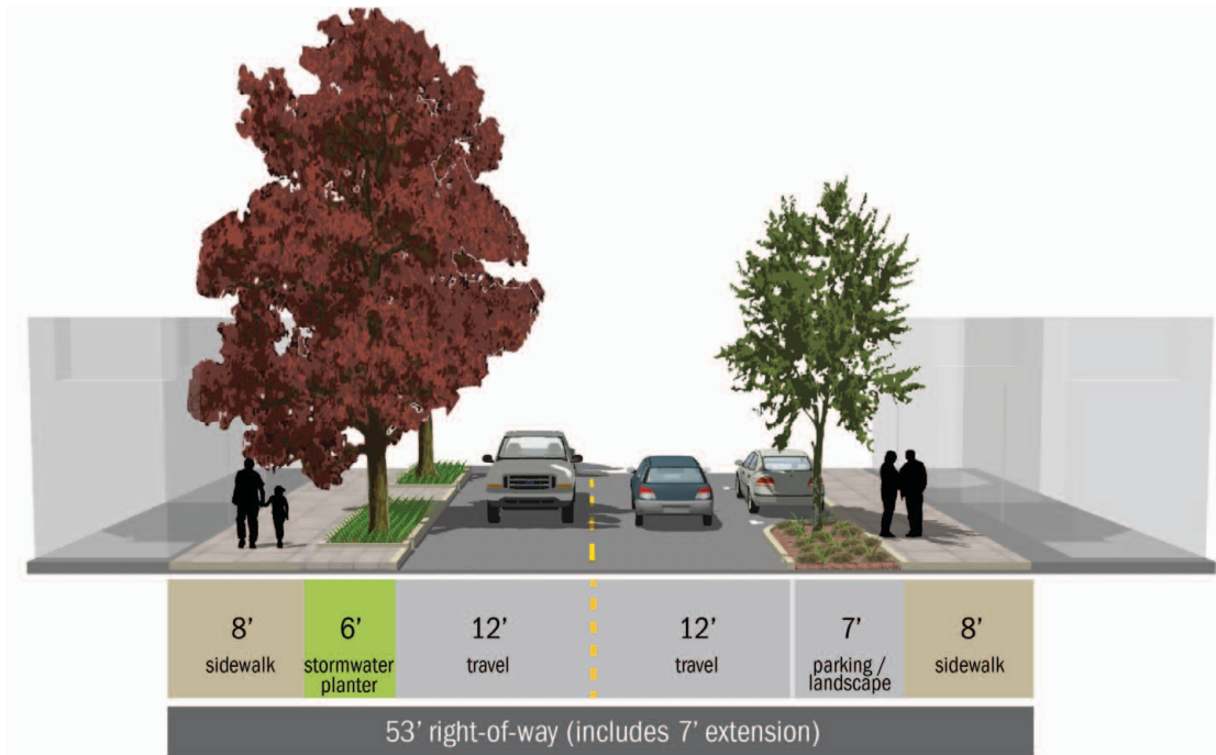
Figure A-7. Conceptual Cross-Section for Main Street – North of Beta Street with additional right-of-way
