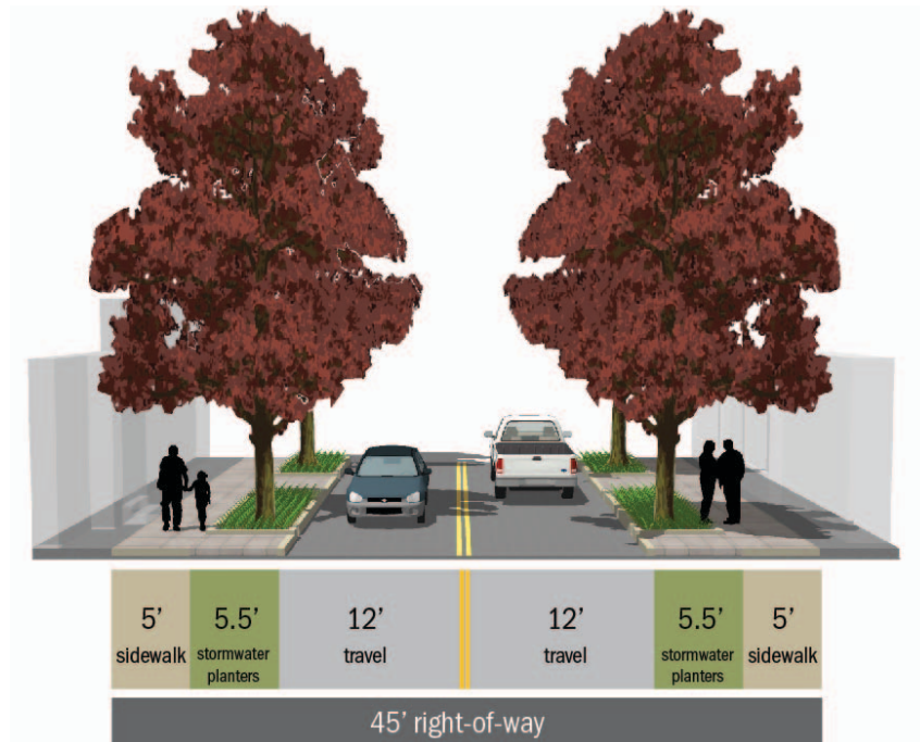
Figure A-10. Conceptual Cross-Section for Ochoco Street – East of Main Street within existing right-of-way
