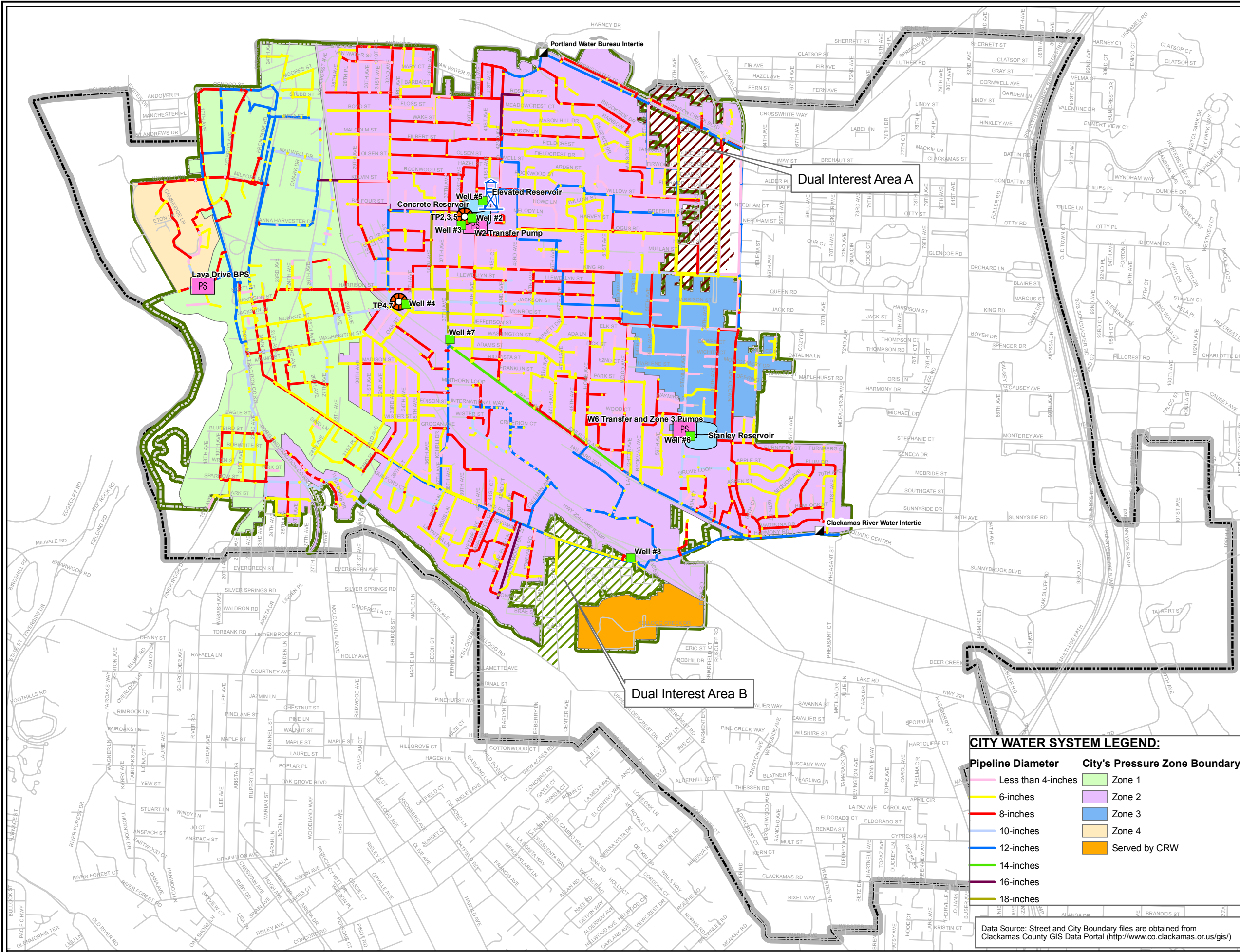
FIGURE 3-1 City of Milwaukie 2010 Water System Master Plan 2010 WATER SYSTEM
