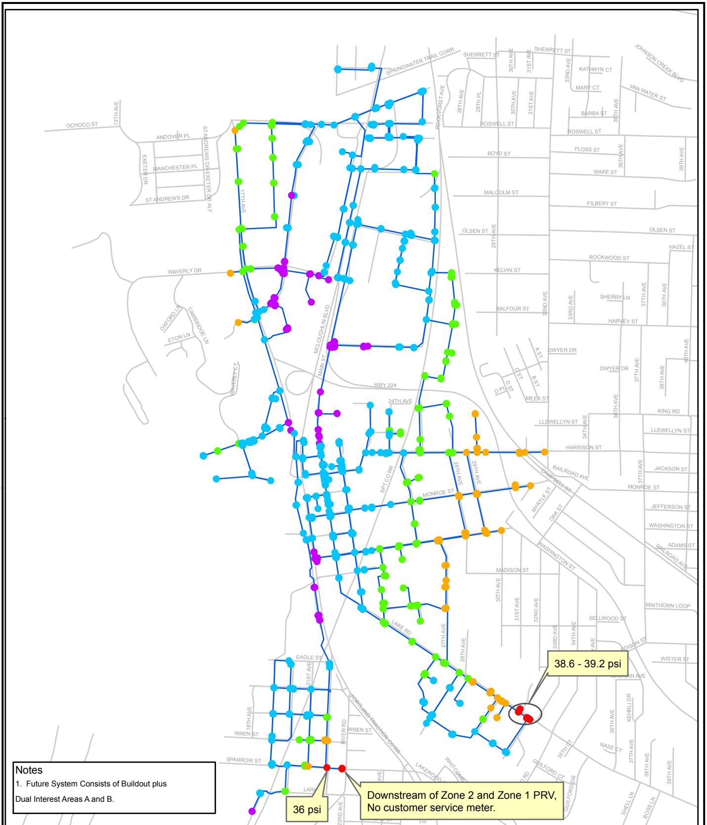
FIGURE 8-4 City of Milwaukie 2010 Water System Master Plan PRESSURE ZONE 1 PEAK HOUR ANALYSIS
