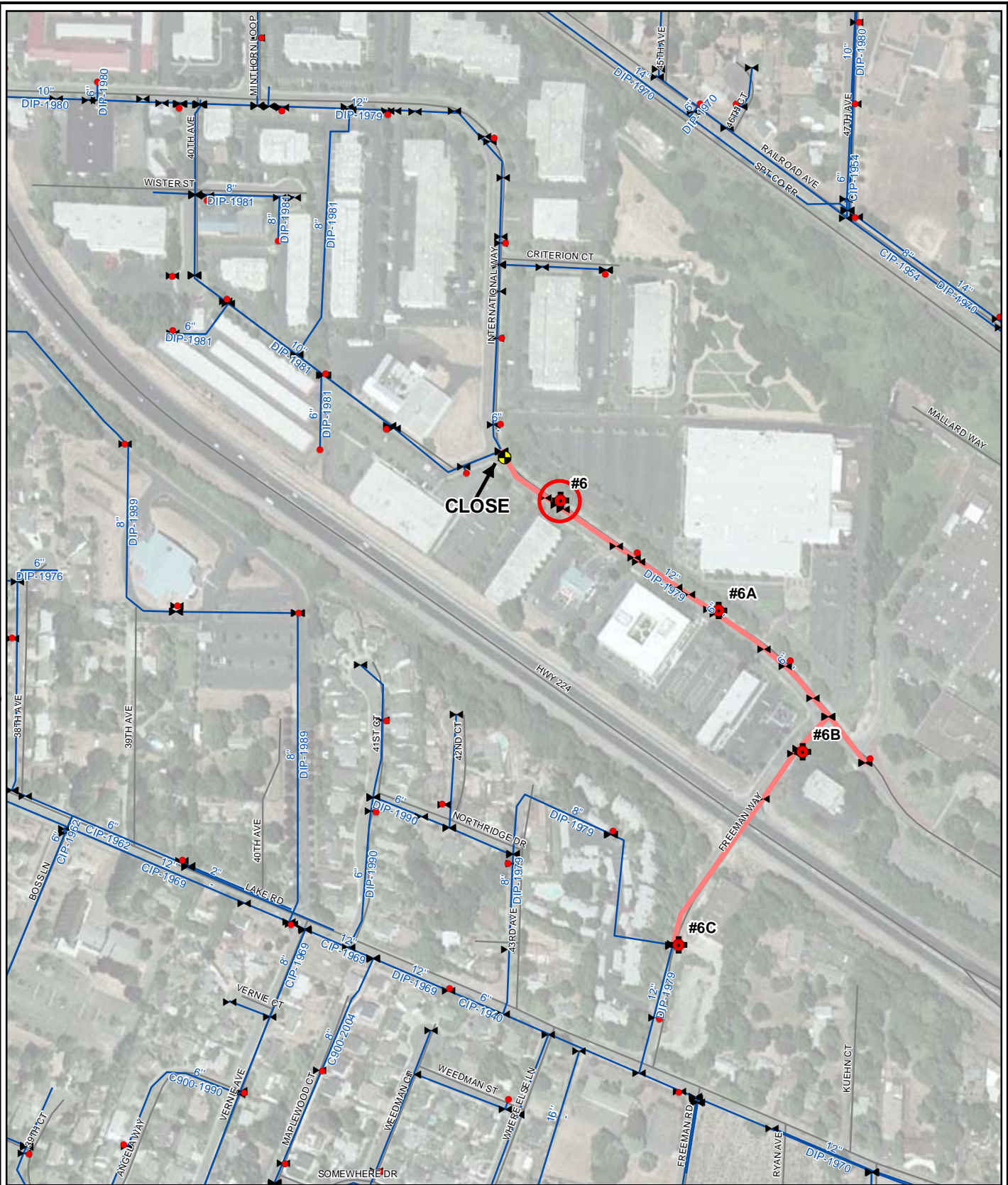
FIGURE A-6 City of Milwaukee Water System Master Plan TEST #6 (12" DIP 1979)
