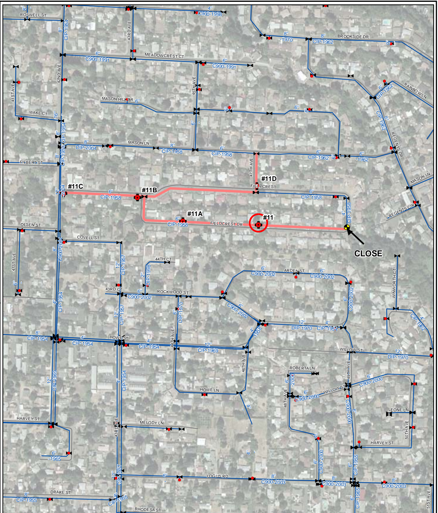
FIGURE A-11 City of Milwaukee Water System Master Plan TEST #11 (6" CIP 1958)
