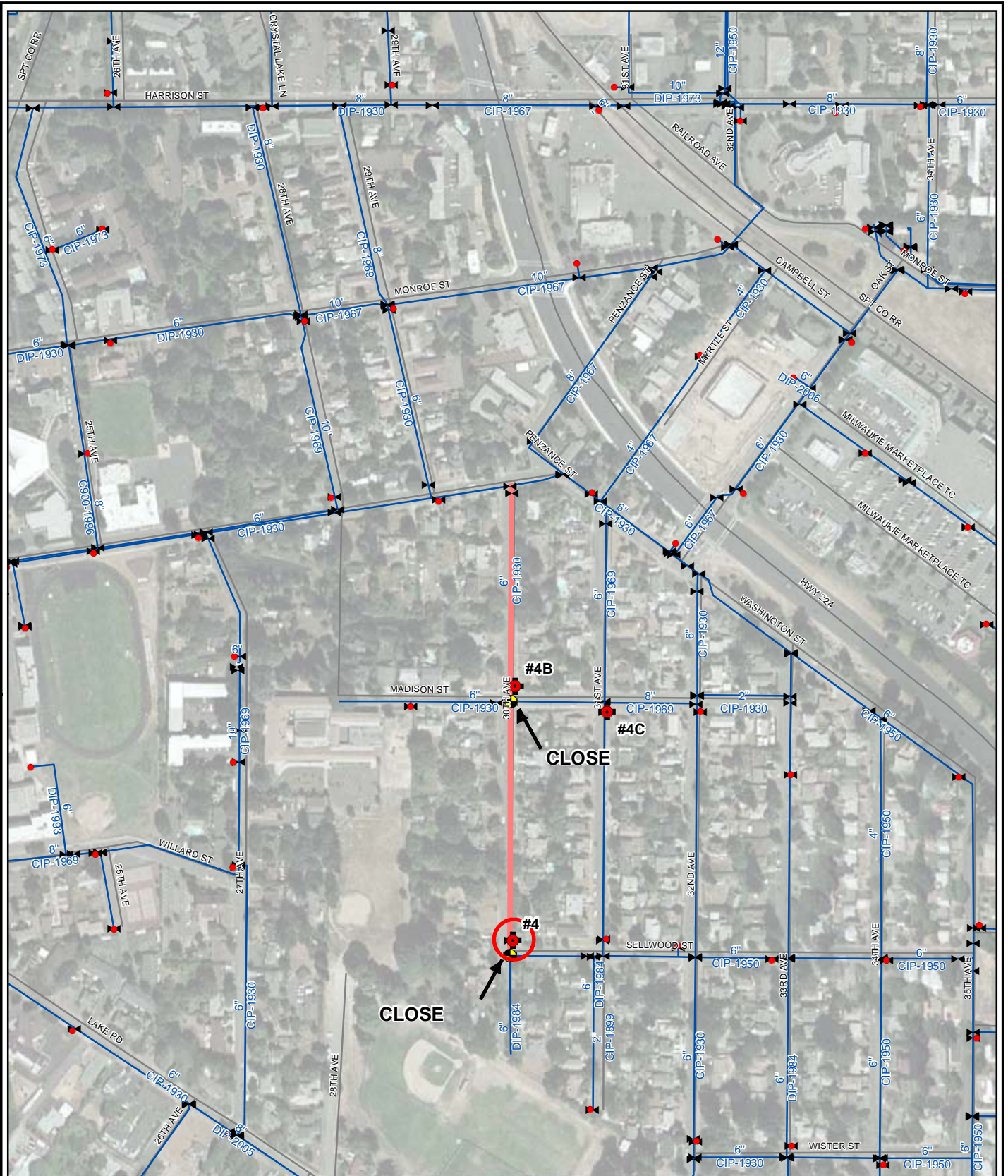
FIGURE A-4 City of Milwaukee Water System Master Plan TEST #4 (6" CIP 1930)
