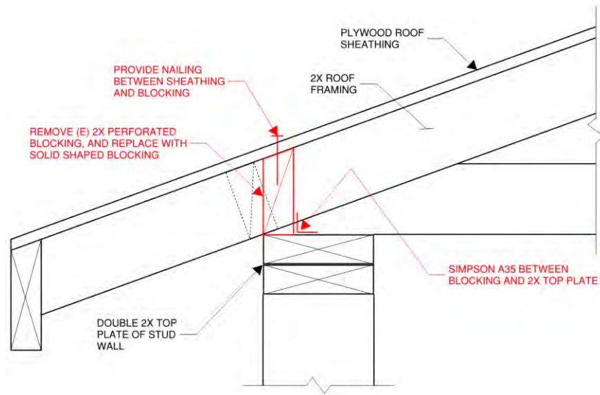
Figure 3.28 – Solid Blocking Between Diaphragm and Shear Wall
