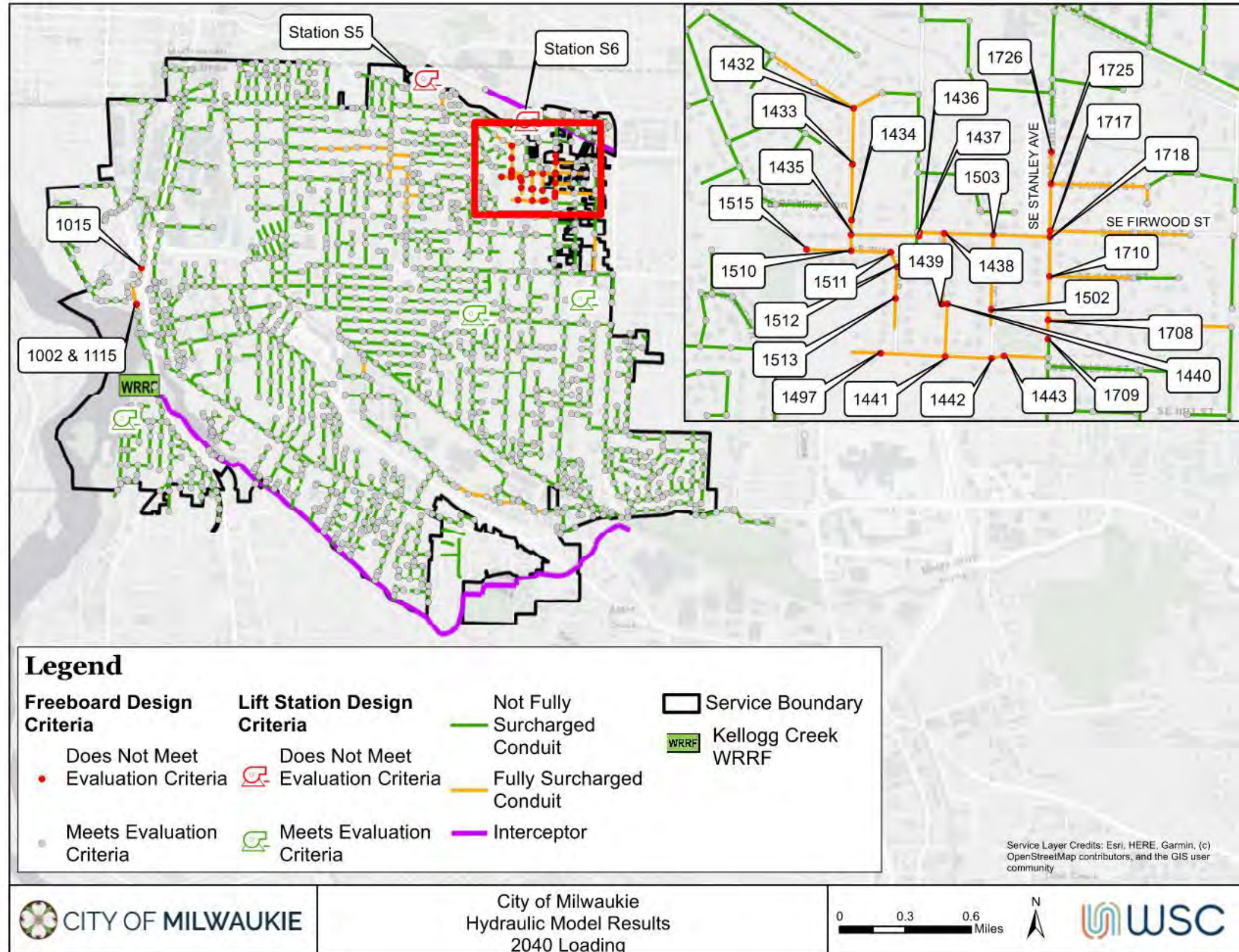
Figure 7-2: Hydraulic Capacity Evaluation Results Under 2040 Loading
