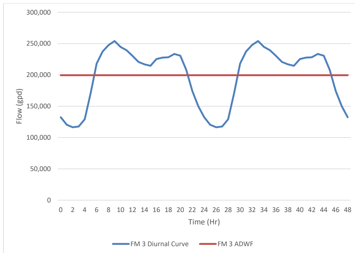
Figure 5-3: Diurnal Curve for Flow Monitor 3
