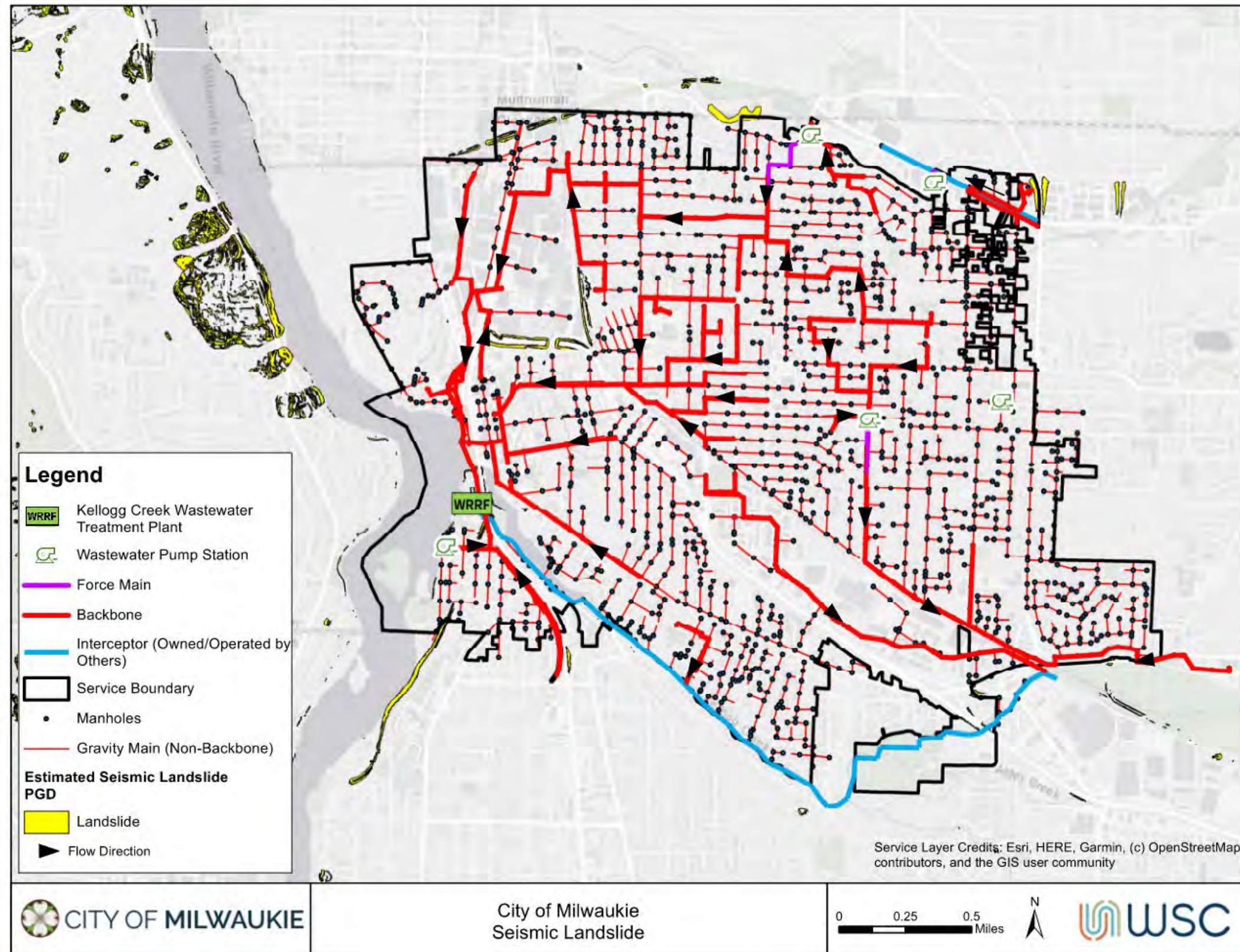
Figure 9-5: Seismic Landslide PGD for M9.0 CSZ Earthquake
