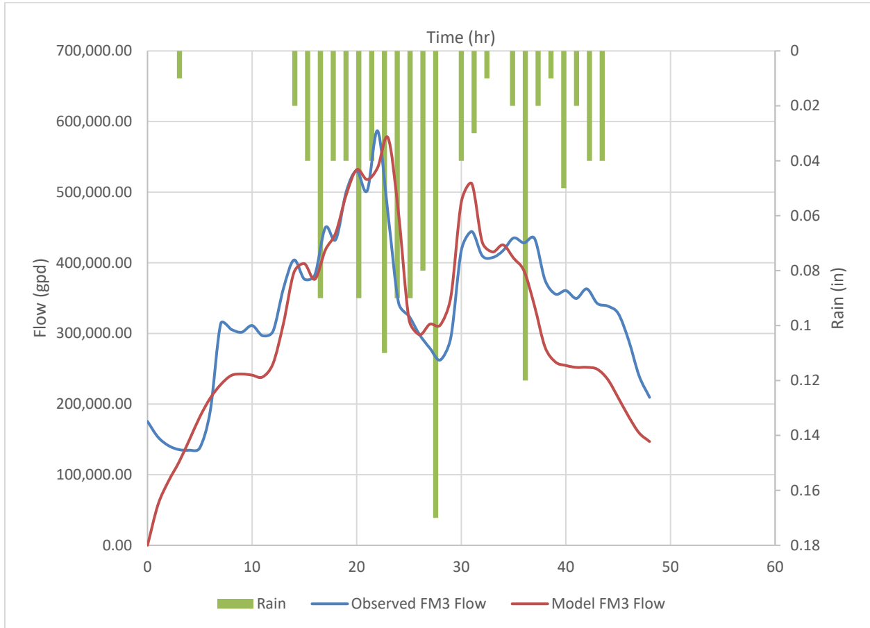
Figure 6-7: Wet Weather Hydrograph at FM 3 During January 27-28 Storm
