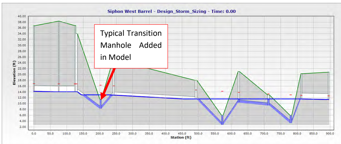
Figure 6-3: Modeling Siphons
