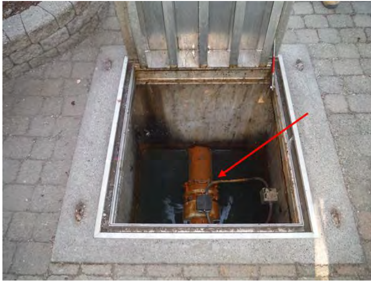
Figure 3.24 – Flowmeter Vault
