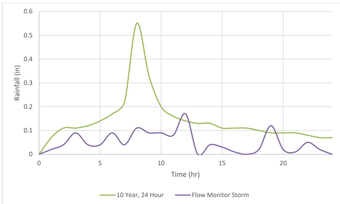
Figure 5-5: Comparison of Storm Hyetographs
