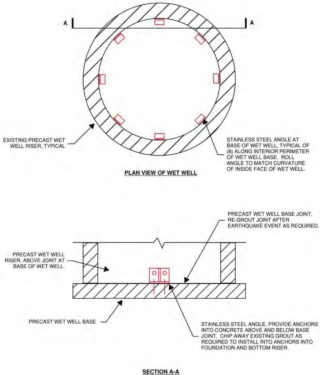
Figure 3.6 – Precast Riser Joint at Foundation Strengthening Concept
