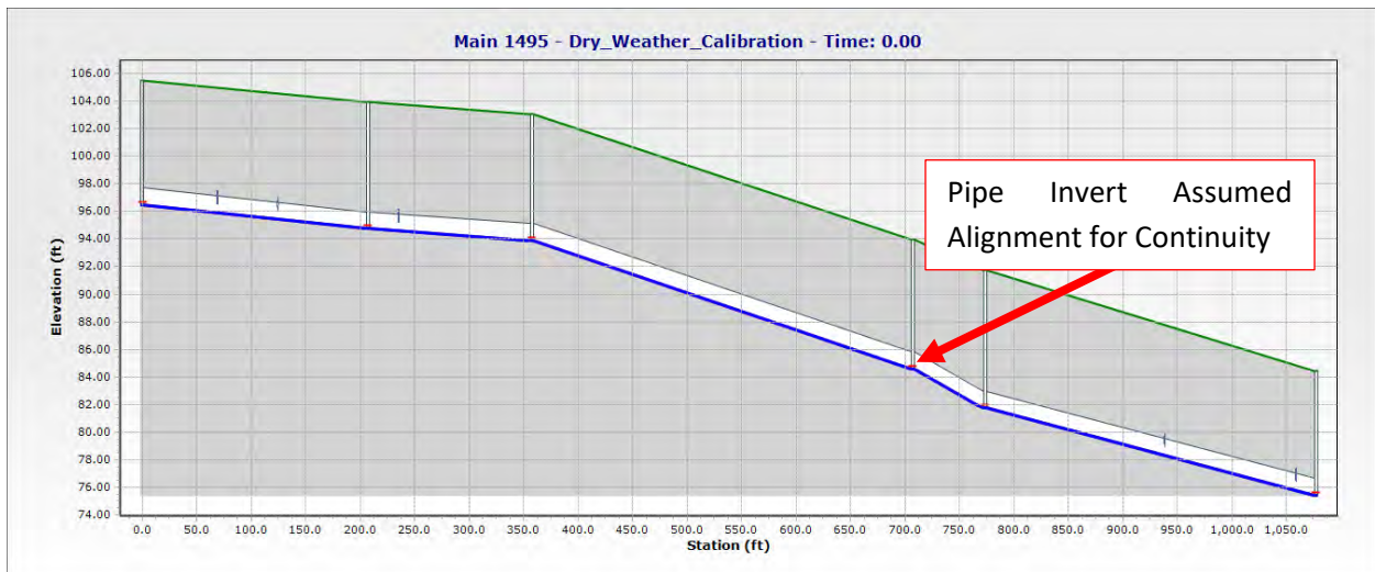
Figure 6-2: Sample Segment with Corrected Connectivity
