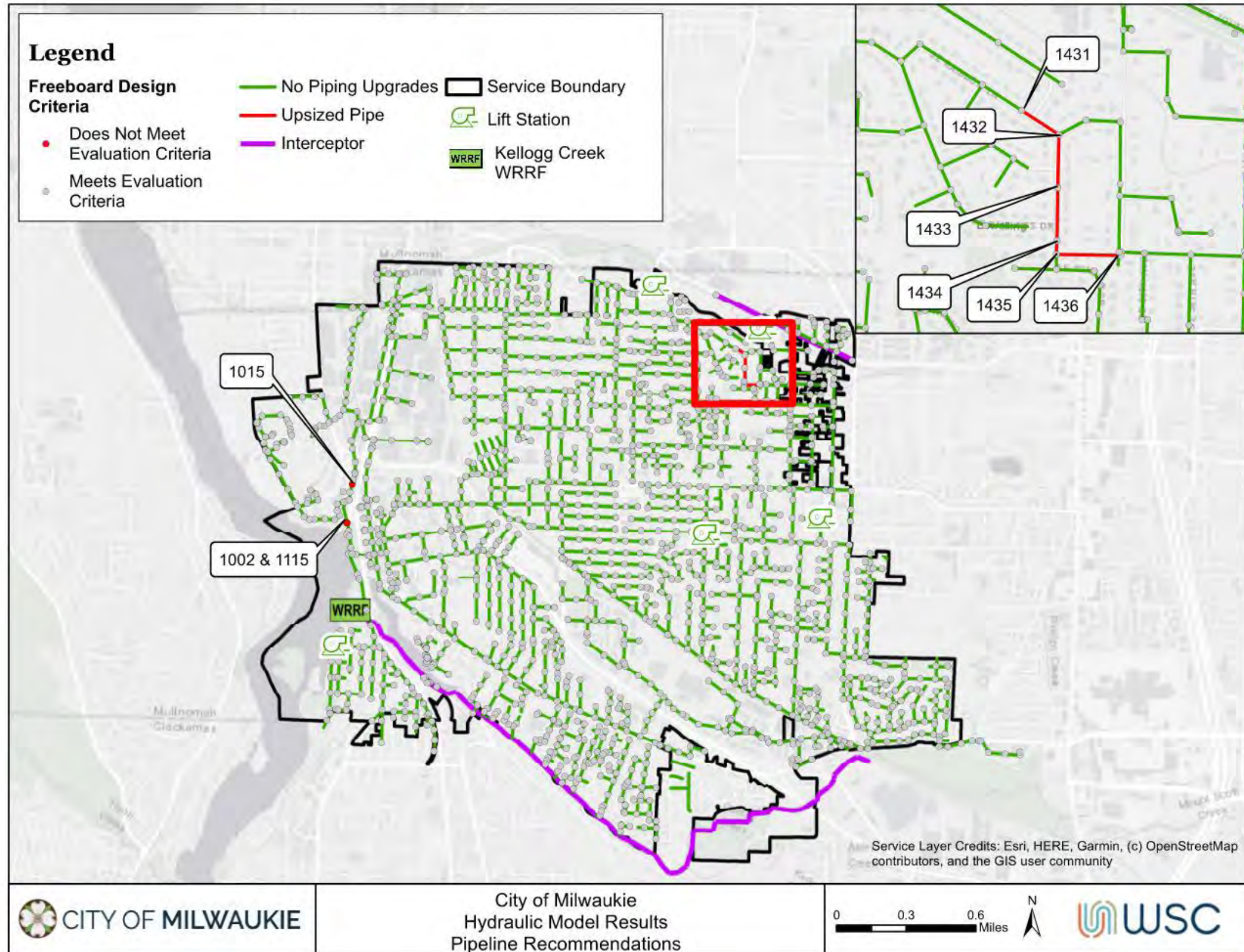
Figure 7-4: Recommended Pipeline Projects
