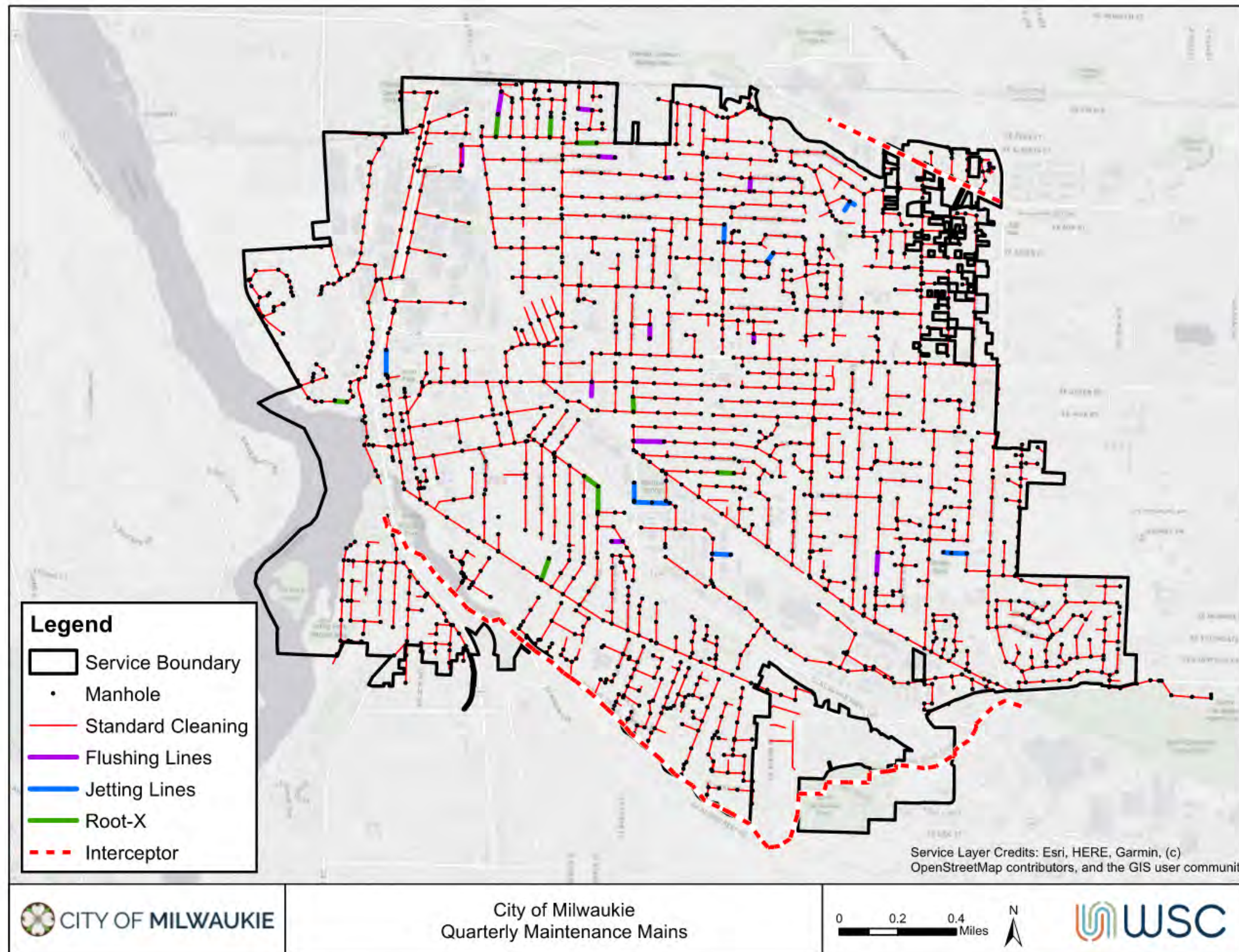
Figure 3-5: Mains Requiring Quarterly Maintenance
