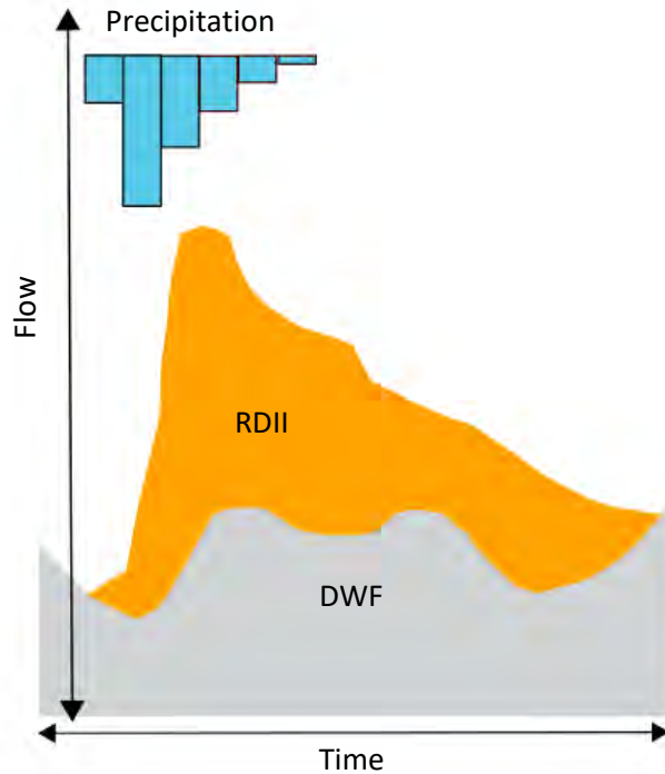
Figure 5-1: Components of Wastewater Flow (15)
