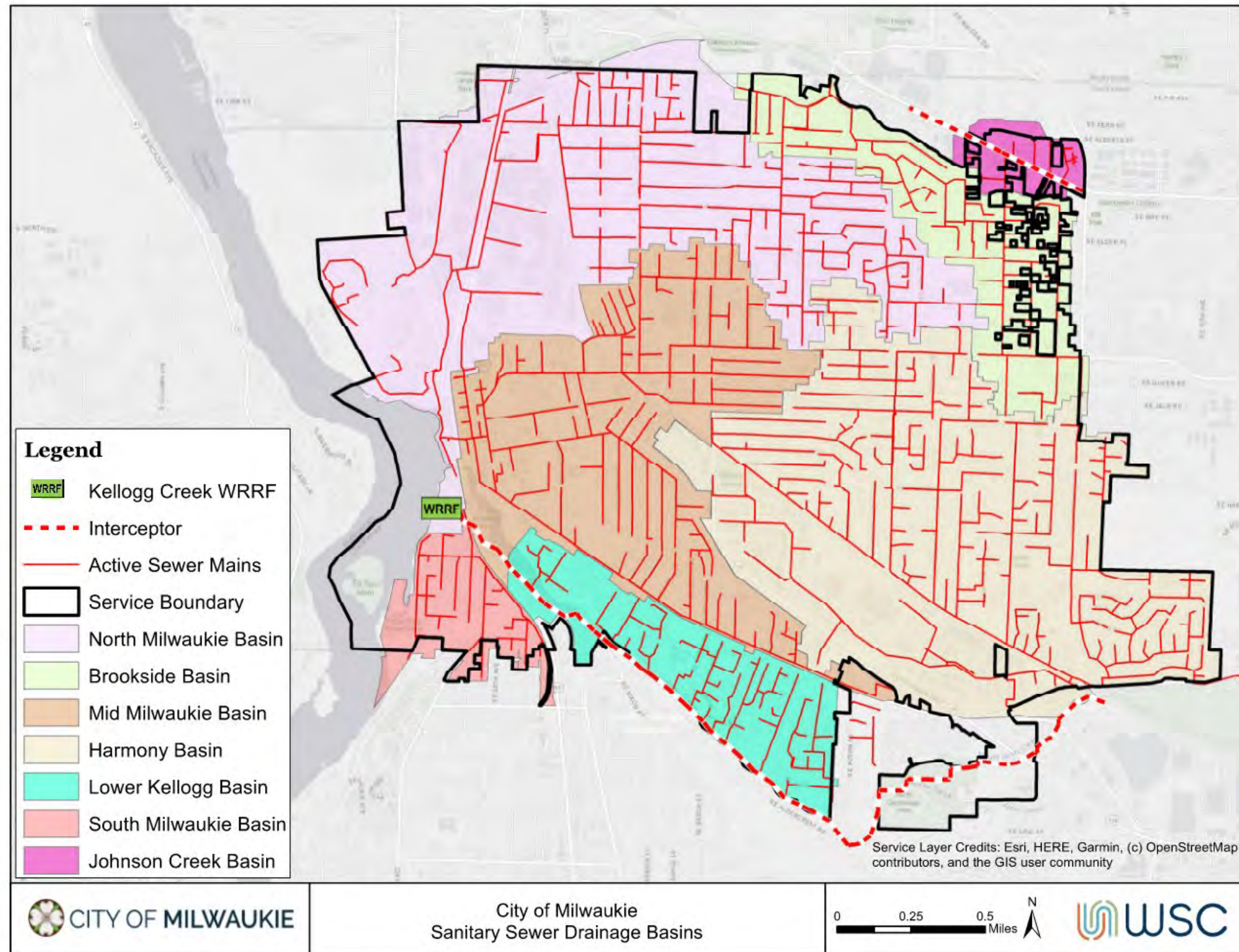
Figure 3-2: Collection System Sewer Basins
