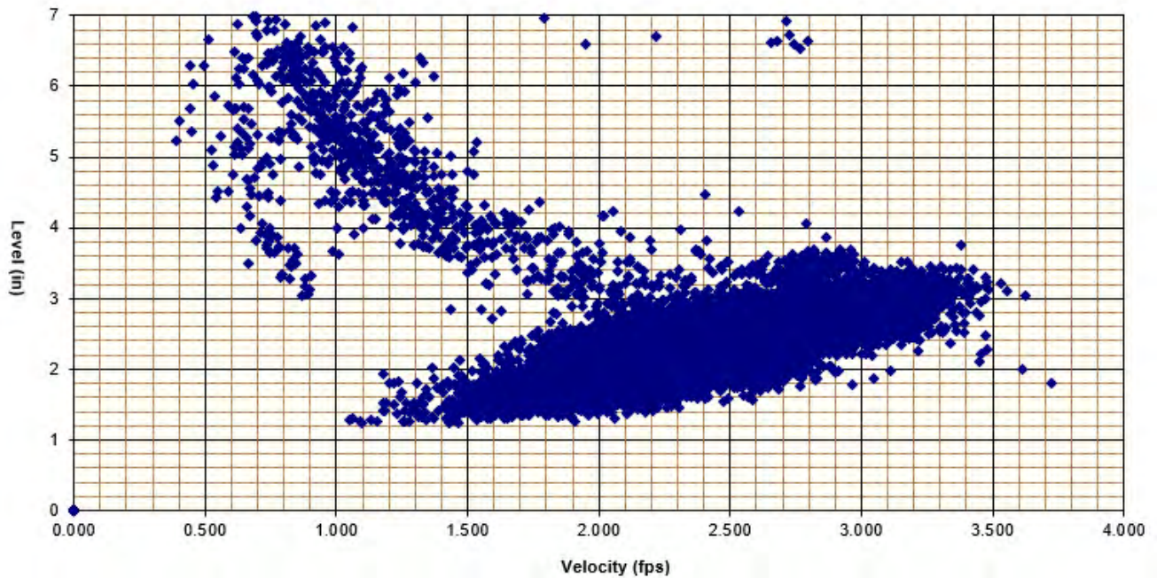
Figure 5-1: Plot of Level versus Velocity for FM 1 between November 2019 and February 2020
