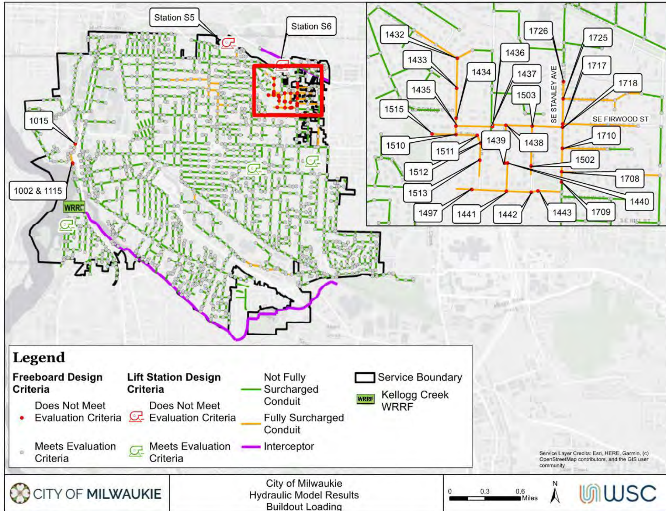
Figure 7-3: Hydraulic Capacity Evaluation Results Under Buildout Loading
