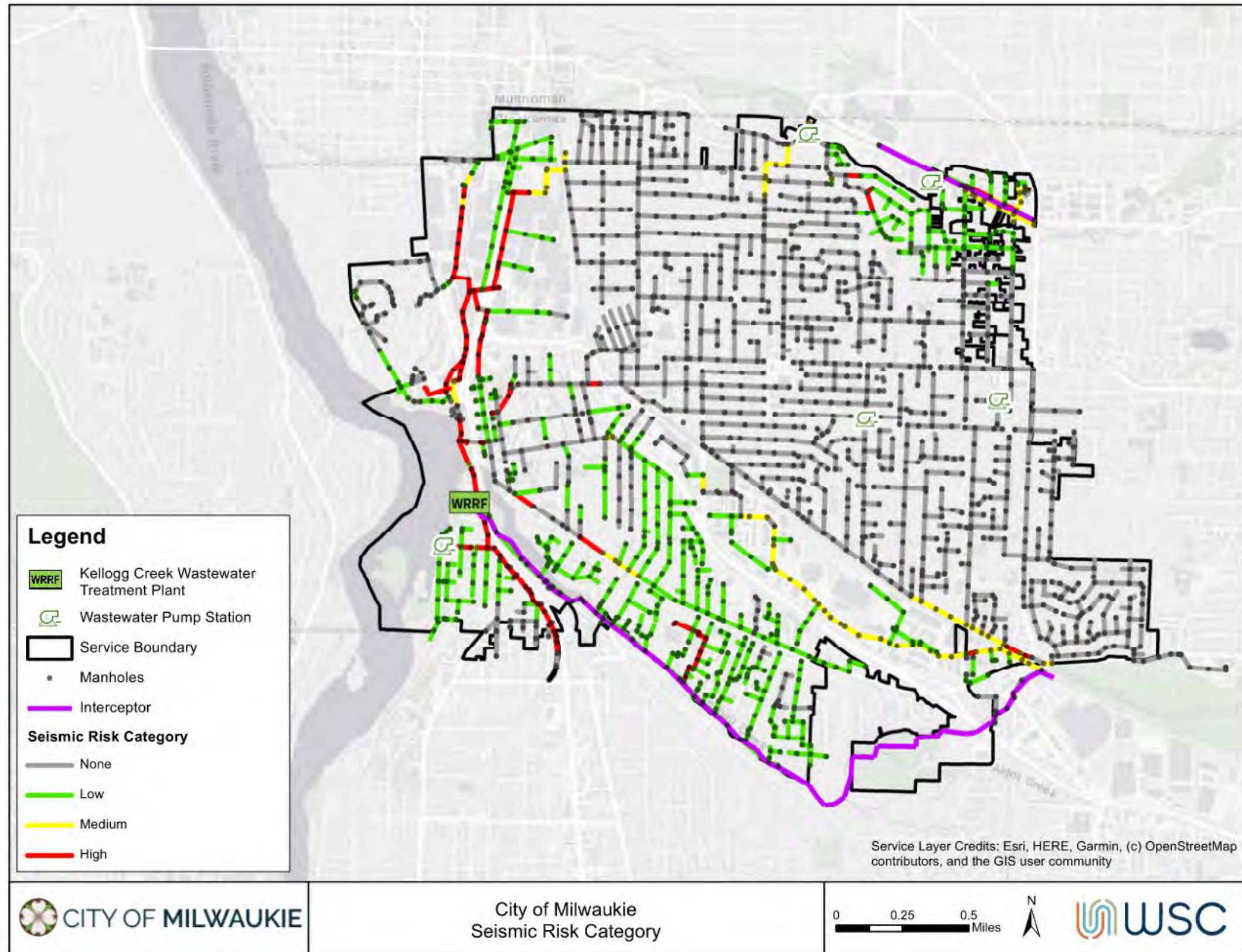
Figure 9-8: Seismic Risk Prioritization
