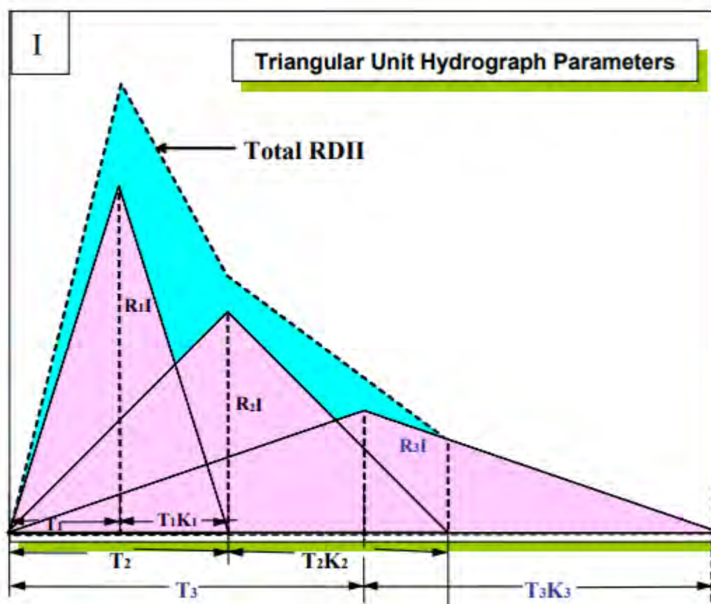
Figure 5-4: RTK Unit Hydrograph Parameters (15)
