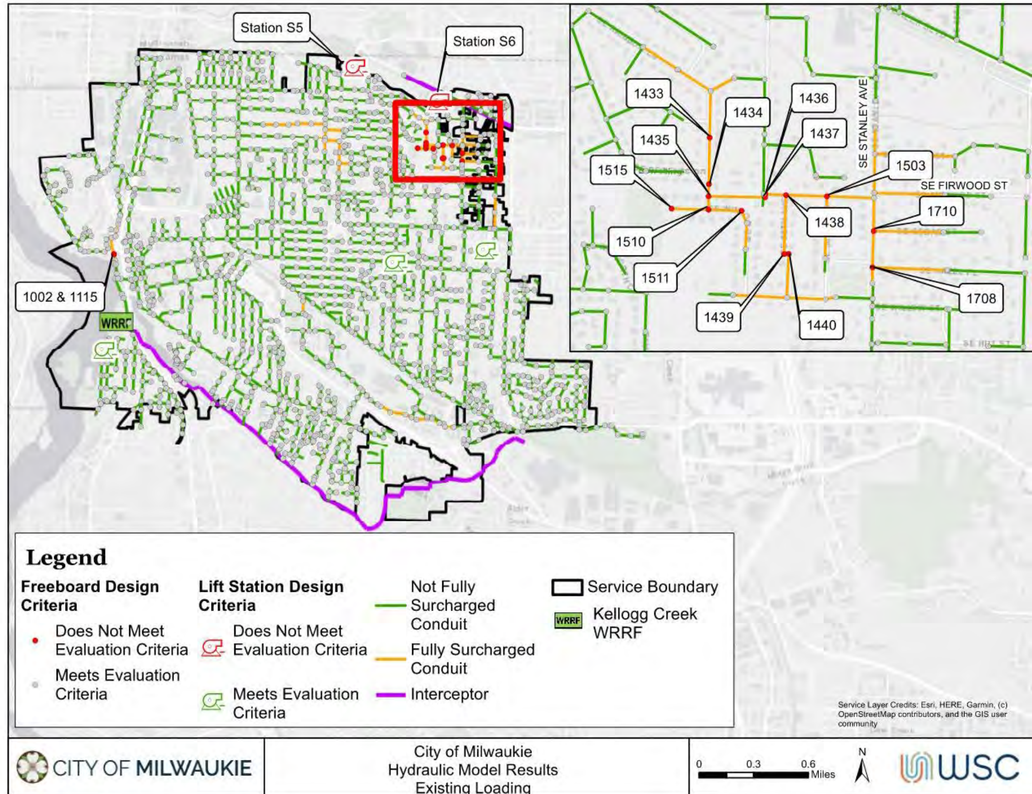
Figure 7-1: Hydraulic Capacity Evaluation Results Under Existing Loading
