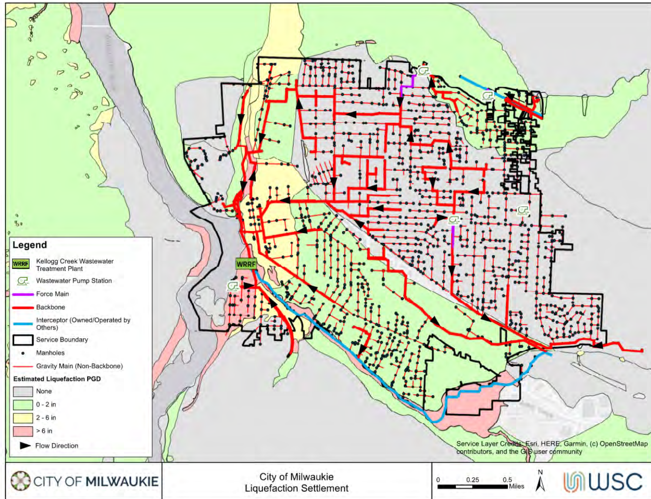
Figure 9-3: Liquefaction Settlement PGD for M9.0 CSZ Earthquake
