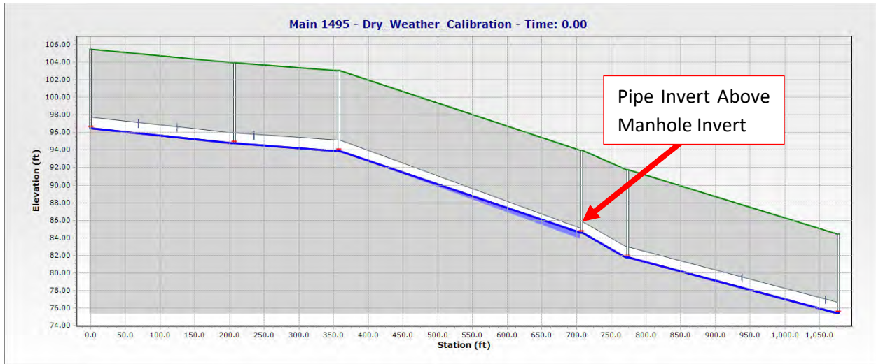
Figure 6-1: Sample Segment with Connectivity Issue
