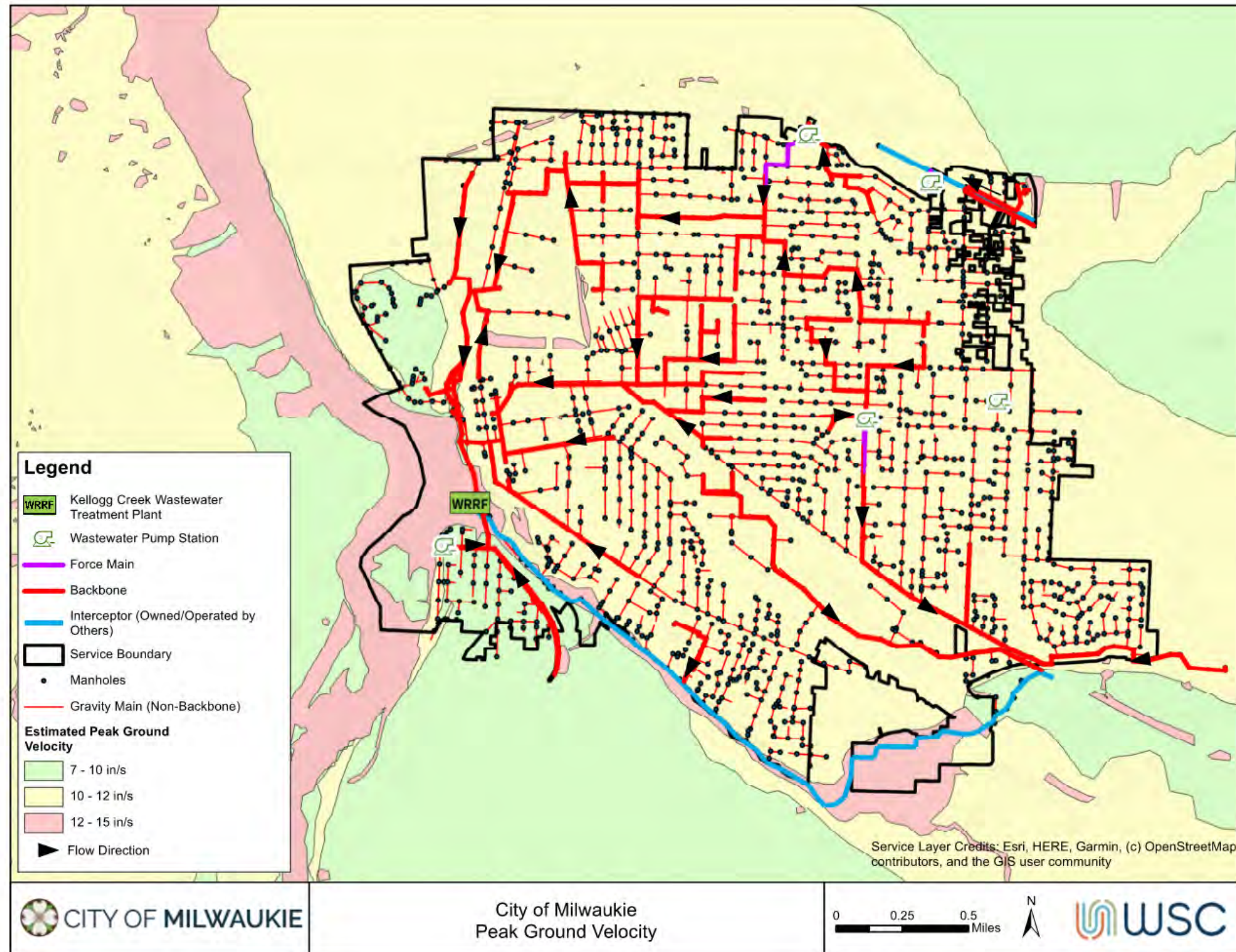
Figure 9-2: Peak Ground Velocity for M9.0 CSZ Earthquake
